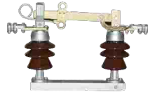
GOAB Switch
